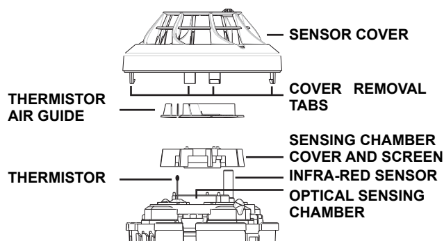
Figure 6: Cleaning the Sensor
