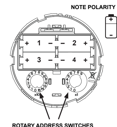
Figure 4: Battery Installation and Rotary Address Switches
