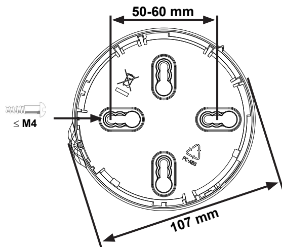
Figure 1: B501RF Mounting
